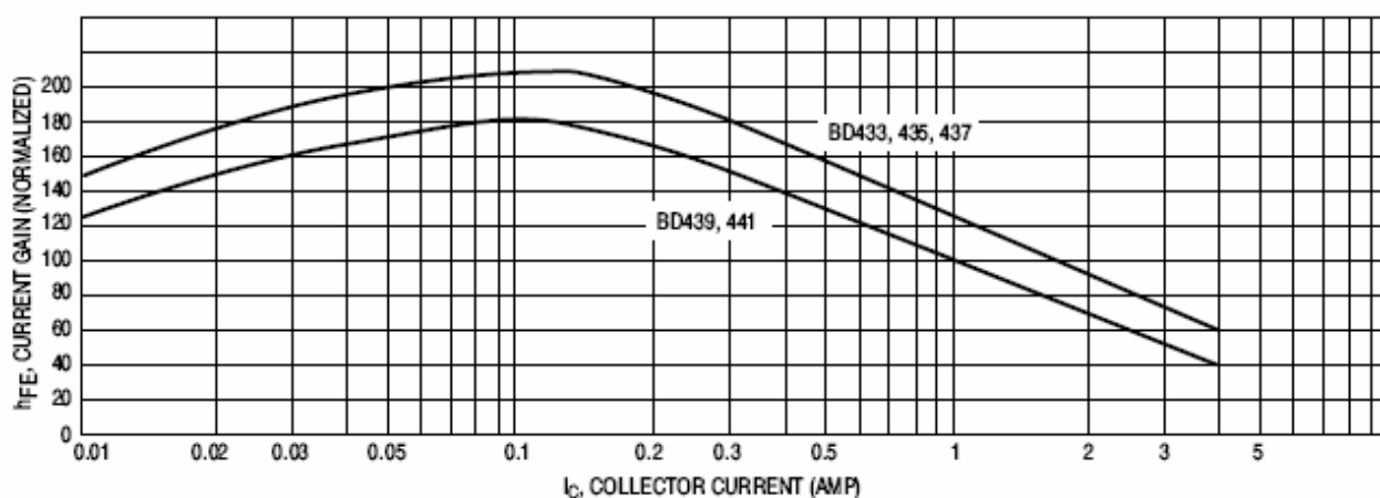
Figure 2. Current Gain
